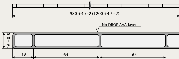
Section of PLEXIGLAS® Resist AAA SDP 16-64 (dimensions in mm)
