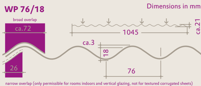
Cross-section of PLEXIGLAS® Heatstop Cool Blue WP 76/18 (dimensions in mm)
