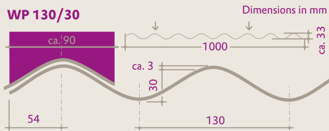
Cross-section of PLEXIGLAS® Resist WP 130/30 (dimensions in mm)
