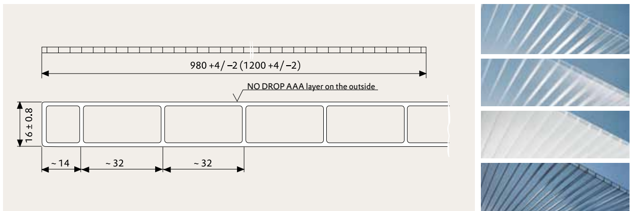
Section of PLEXIGLAS RESIST® AAA SDP 16 (dimensions in mm)
